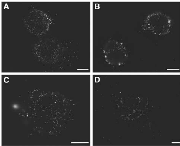
Figure 4 Reorganization of hyaluronan under the cell during spreading. Hyaluronan reorganization is observed by scanning electron microscopy using QX TM capsules. RCJ-P cells were labeled with biotinylated hyaluronan-binding protein and streptavidin-conjugated colloidal gold, and seeded in a QX TM capsules for 5, 10, 20, and 30 min before fixation. Gold particles are visible on the ventral side of the cell membrane (white particles). (A) Gold particles are scattered evenly under the cells 5 min after seeding. (B) After 10 min the gold particles appear more organized within discrete areas under the cells. (C, D) At 20 and 30 min after seeding, the gold particles become increasingly clustered in compartments under the cells. Scale bars = 5 \mu\text{m} .
